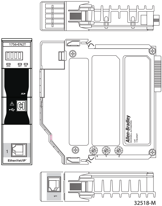
Figure 1 - 1756-EN2T
