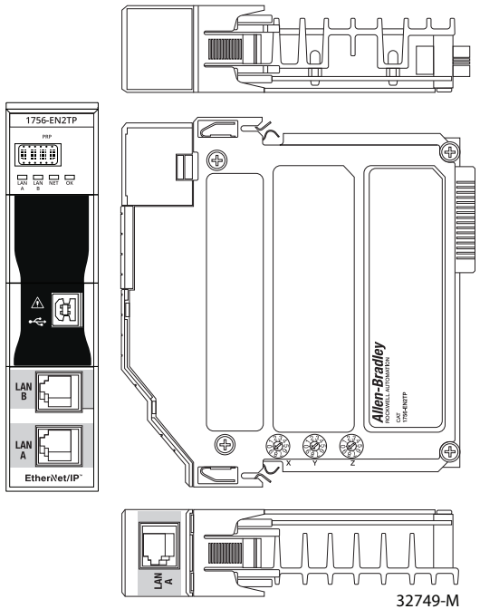
Figure 2 - 1756-EN2TP
