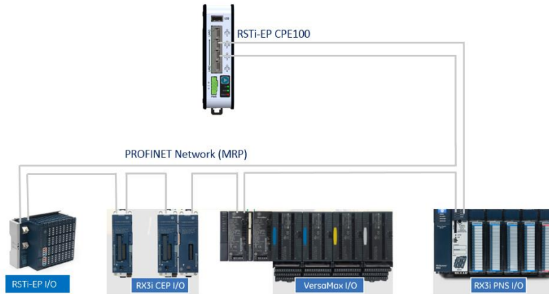
Figure 25: Typical Multi-Tier LAN Application (Ring Topology)
