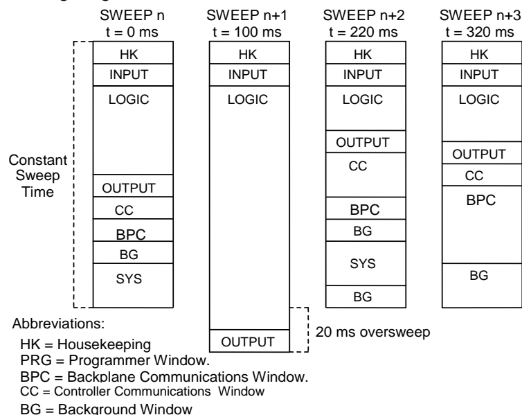
Figure 32: Typical Sweeps in Constant Sweep Mode
