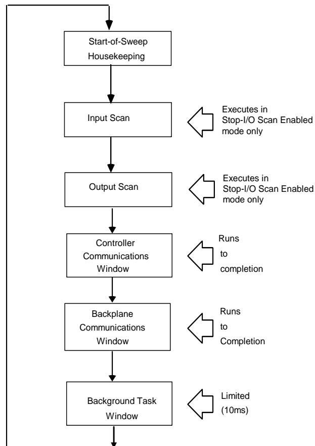
Figure 34: CPU Sweep in Stop-I/O Disabled and Stop-I/O Enabled Modes
