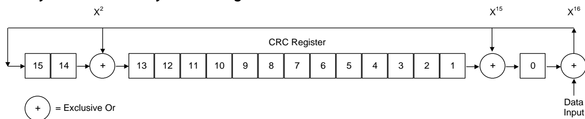
Figure 41: CRC Register Operation
