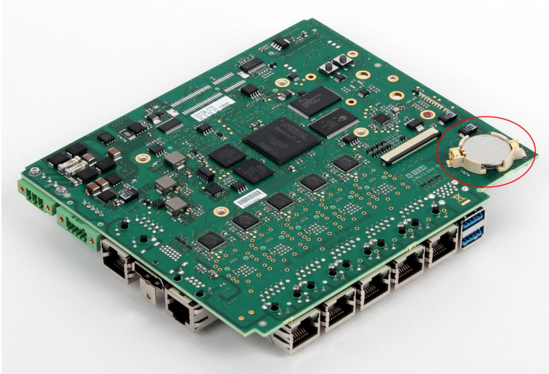
Figure 7: Location of RTC battery on CPE400
