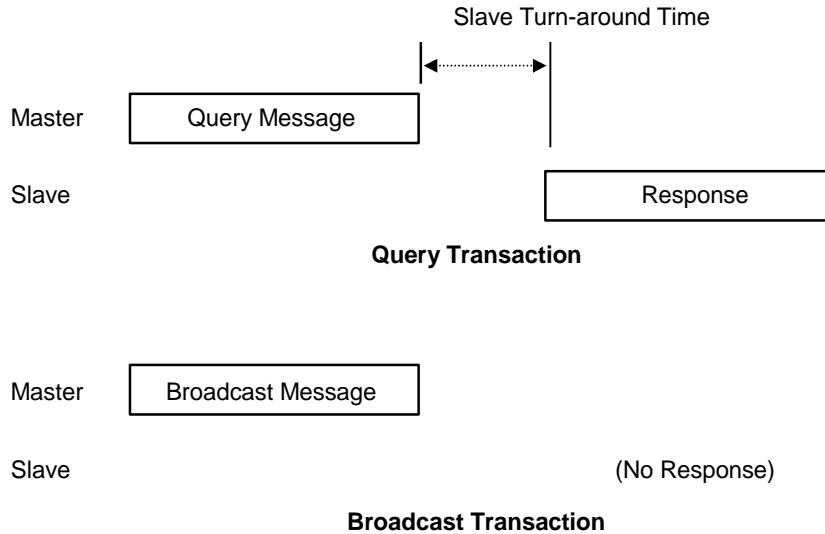
Figure 39: RTU Message Transactions
