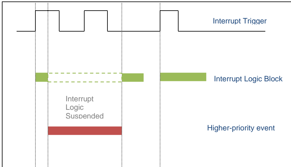
Figure 55: Interrupt Execution Considerations
