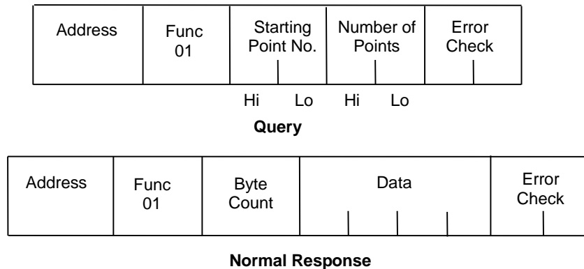
Figure 42: RTU Read Output Table Message Format
