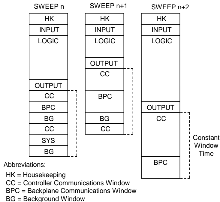
Figure 33: Typical Sweeps in Constant Window Mode
