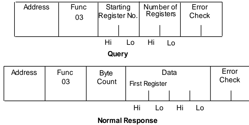
Figure 44: RTU Read Registers Message Format
