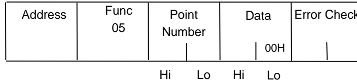
Figure 46: RTU Force Single Output Message Format
