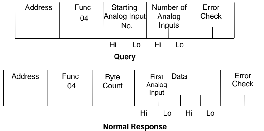
Figure 45: RTU Read Analog Inputs Message Format
