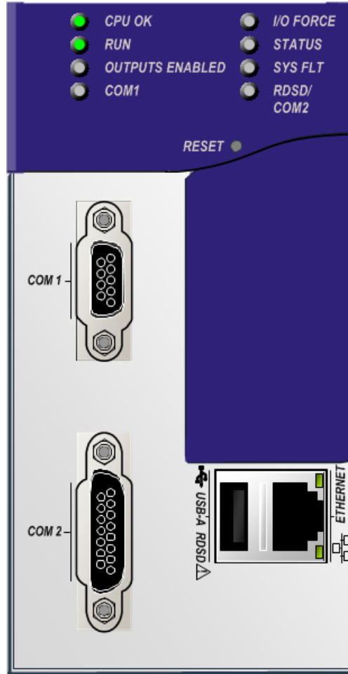
Figure 14: IC695CPE310 Front View
