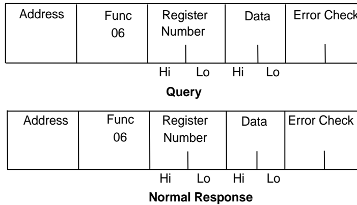
Figure 47: RTU Preset Single Register Message Format
