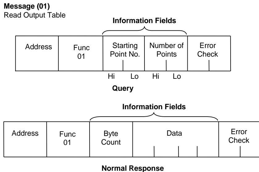
Figure 40: RTU Read Output Table Example
