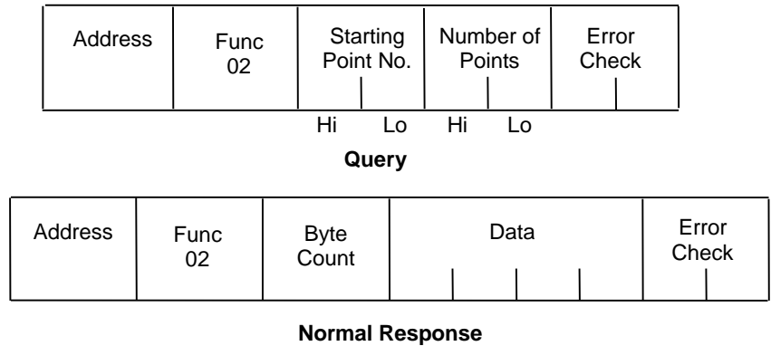
Figure 43: RTU Read Input Table Message Format
