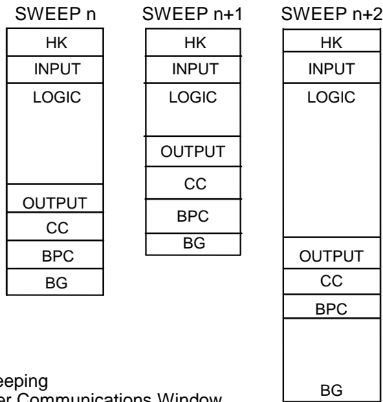
Figure 31: Typical Sweeps in Normal Sweep Mode
