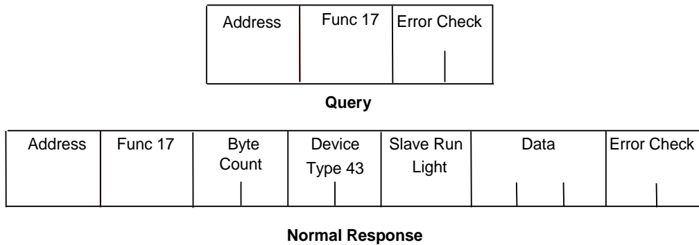
Figure 52: RTU Report Device Type Message Format
