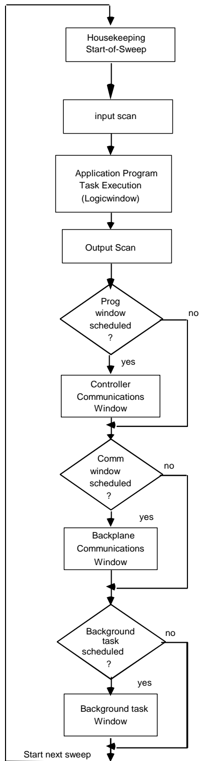
Figure 30: Major Phases of a Typical CPU Sweep
